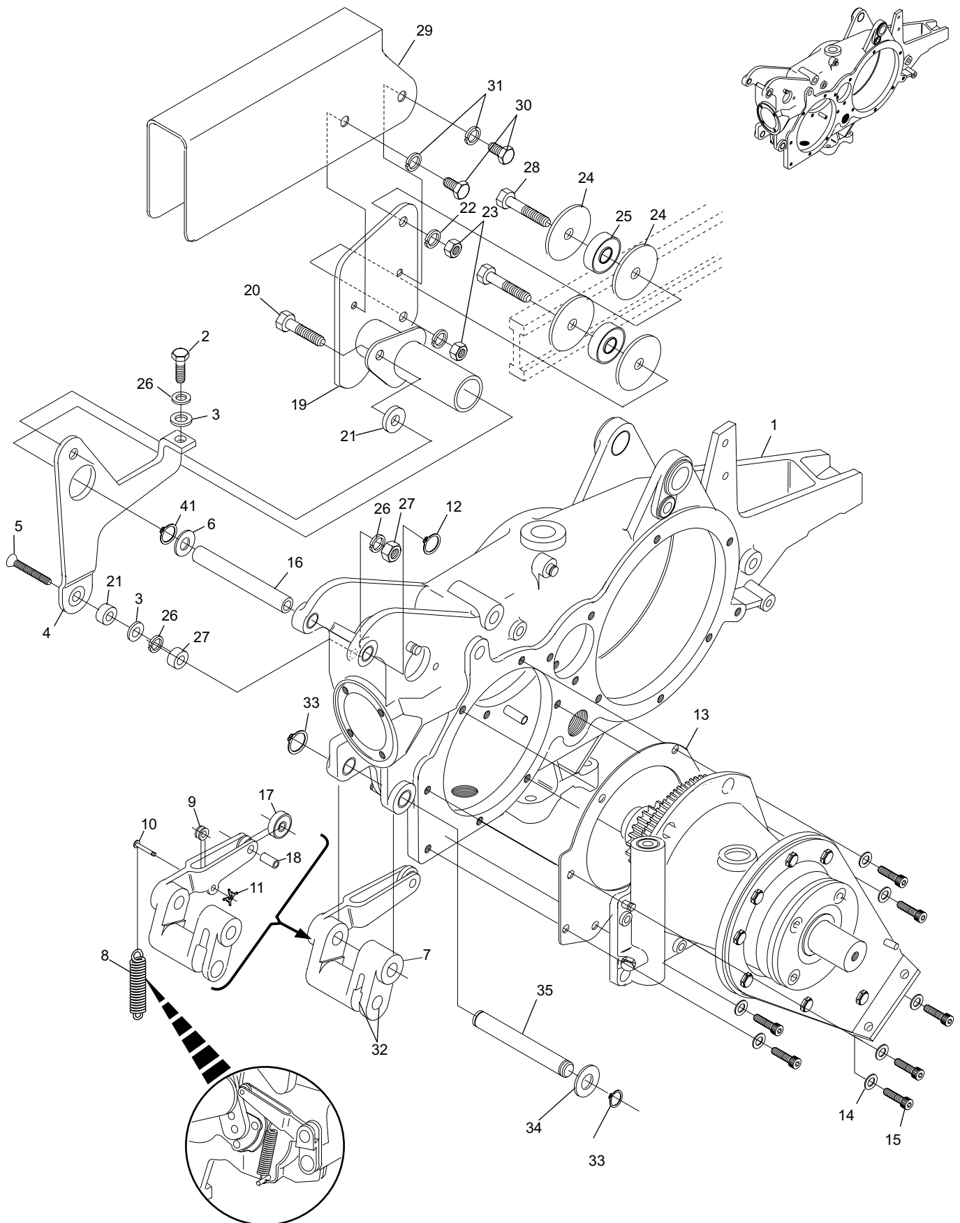
Gear Box Assembly
