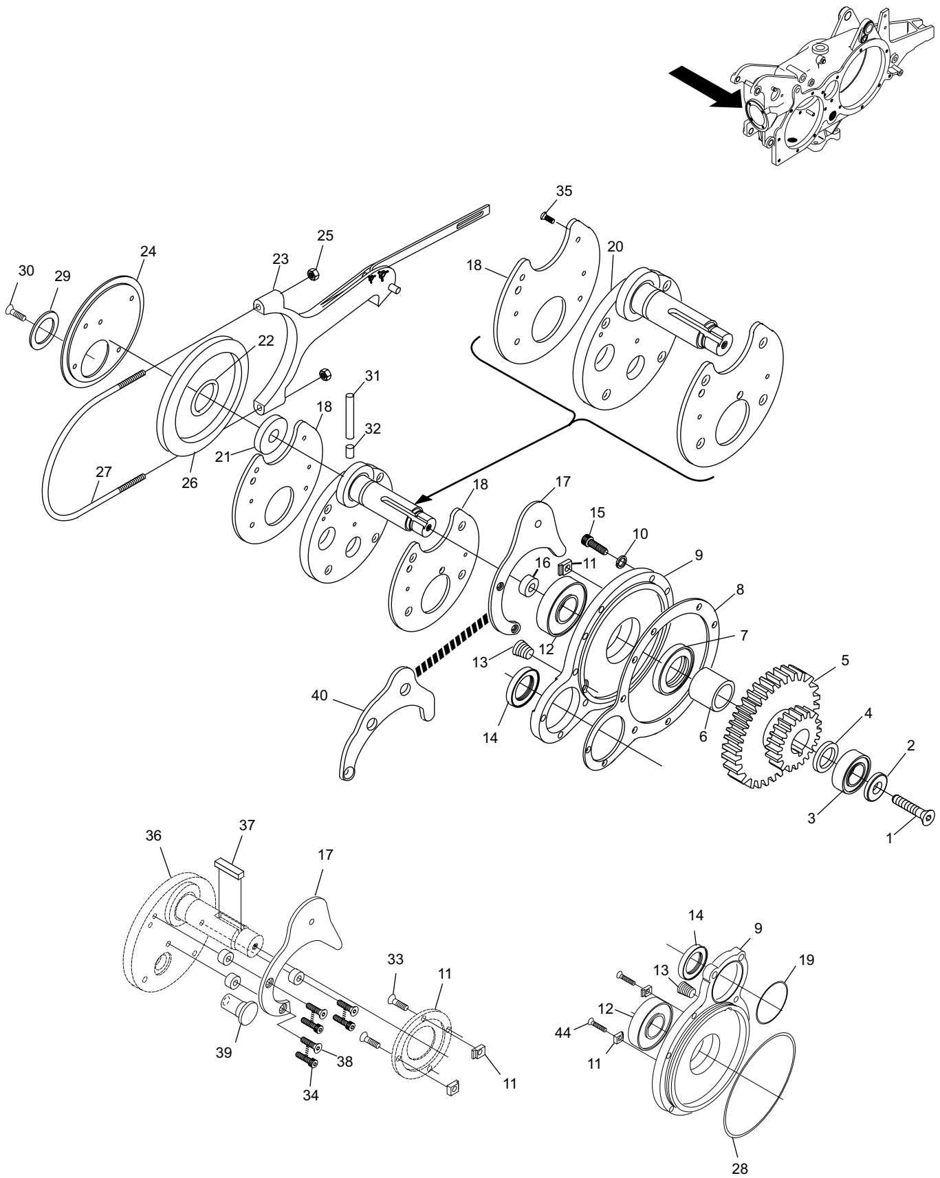
Deck Lift Crank Assembly For "A", "A" Converted to A-2 and A-2 w/o Scotch Yoke
