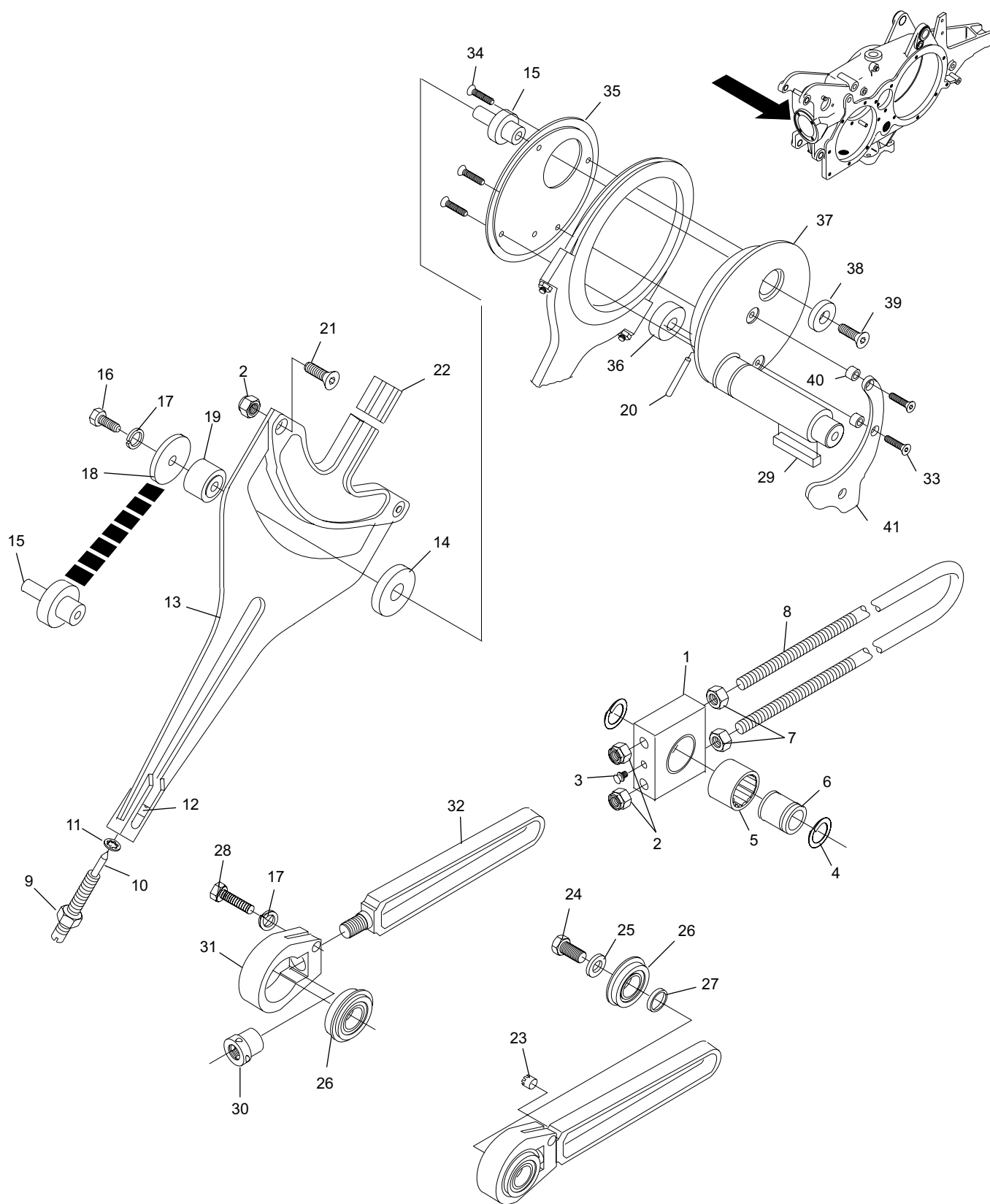
Deck Lift Eccentric Assembly For A-2 w/Scotch Yoke Only
